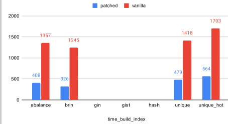
io2, 50 clients (less - better)
