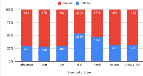
io2, 8 clients, (less - better)
