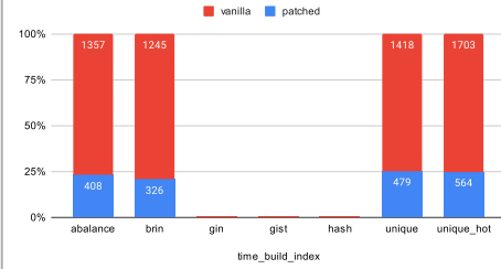
io2, 50 clients (less - better)
